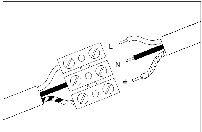
4. Connect the 3 power wires according to their colours. Brown is the live wire, blue is the neutral wire, the green yellow wire is the earthwire.
