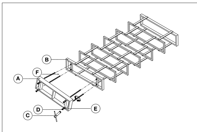
1. Assemble the base to the cabinet.
