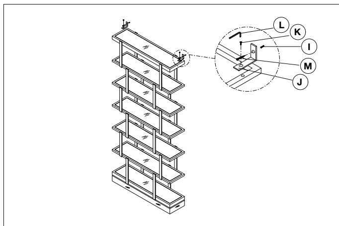
3. Install part (J) and fix the cabinet to the wall to prevent it from tipping over.
