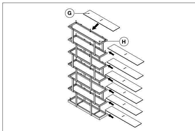
2. Place the glass.
